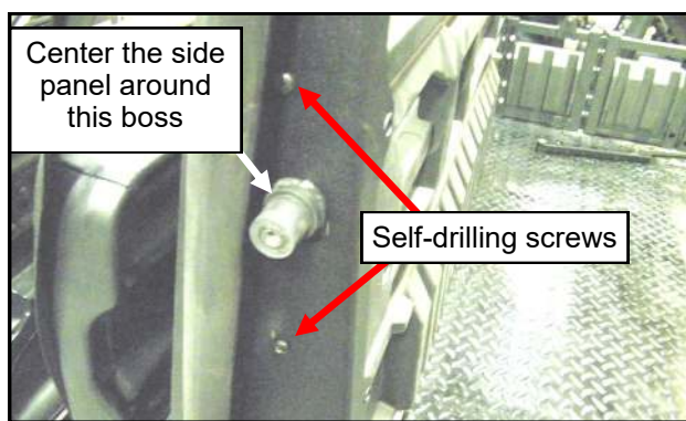
Fig. 3.2 Rear panel sides
