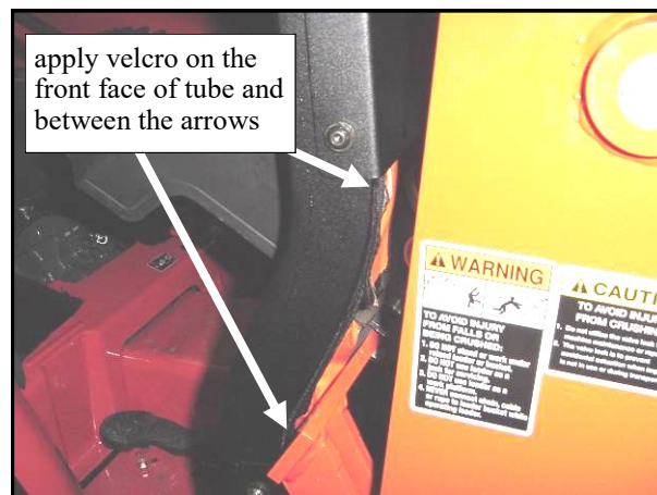
Fig. 15.1a (view from right front side of tractor)
