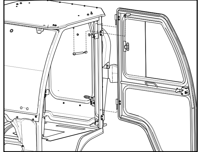
Fig. 19.1 (Door Installation)
