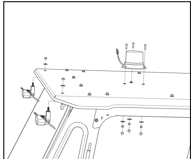
Fig. 1.4 (Remove accessories from roof)
