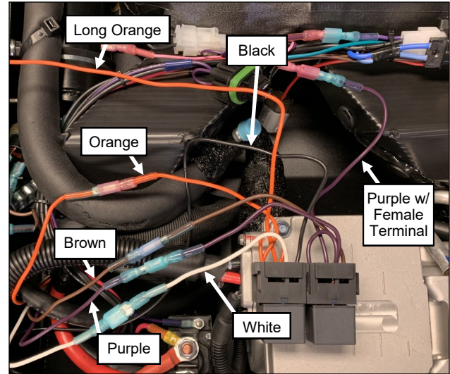
Fig. 2.10 (Connect Controller Wire Harness)
