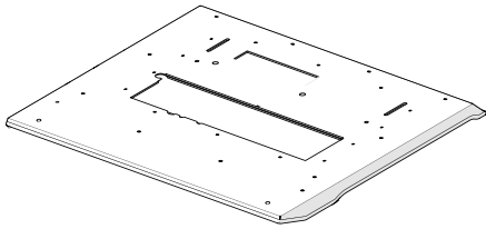
ROOF ASSEMBLY W/ A/C OPENING P/N: 8SV-101-00051
