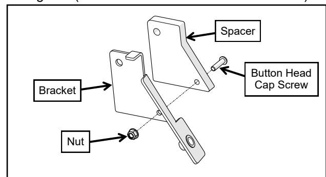
Fig. 1.10 (Install Spacer to Bracket)
