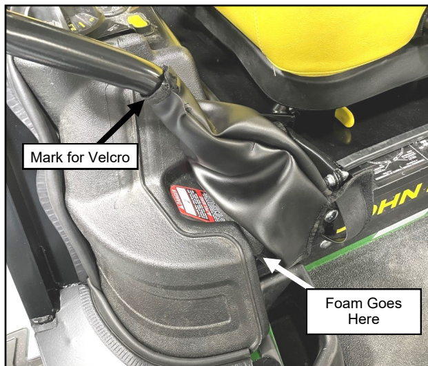
Fig. 2.21 (Loosely Install Drive Handle Filler, Right)
