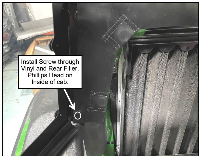
Fig. 2.20b (Attach Rear Filler Vinyl to Right Filler)
