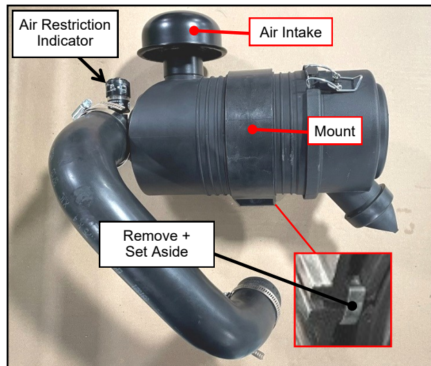
Fig. 2.23a (Reconfigure Air Cleaner, Stock)
