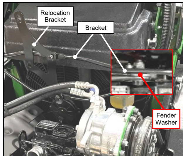
Fig. 2.24 (Install Relocation Bracket)
