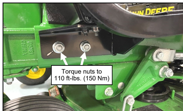
Fig. 2.9 (Tighten Vehicle Frame Bolts, Left)
