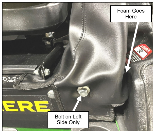
Fig. 2.22 (Install Left Filler, Outside)
