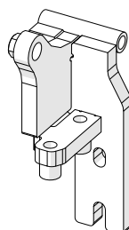
GUARD, BELT P/N: 8SV-SM-02435
