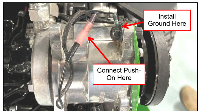
Fig. 2.28b (Connecting AC Harness to Compressor)
