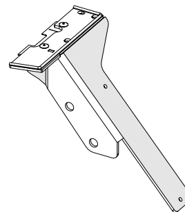
WELDMENT, COMP. TENSIONER P/N: 8SV-WA-00555
