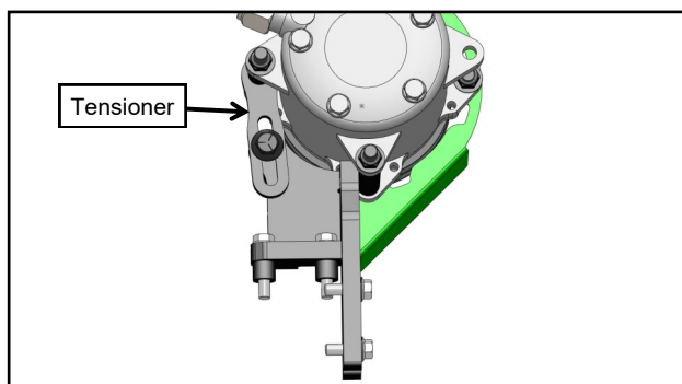
Fig. 2.11b (Install Compressor, Inside View)
