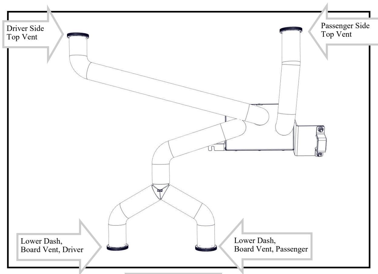
Figure 8.5 Duct Routing
