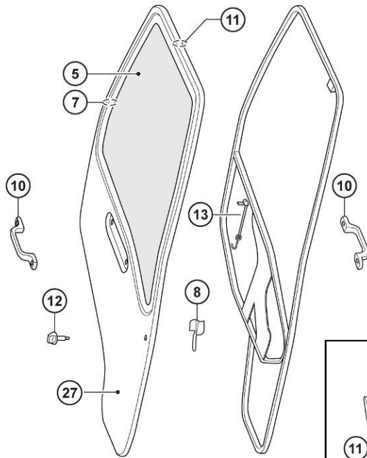
③ Right Outer Door Skin with No Frame Complete
