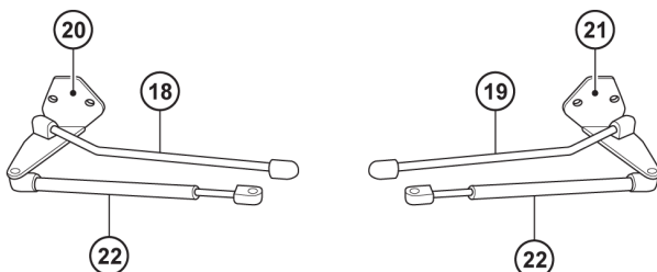
⑳ Top L Hinge Assy Complete ㉑ Top R Hinge Assy Complete
