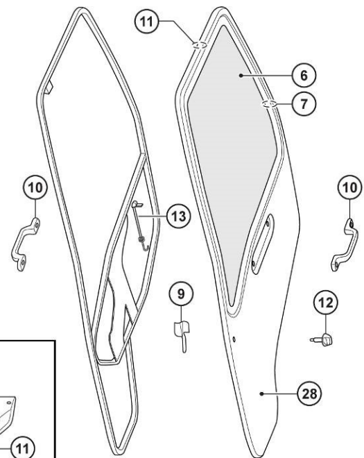
④ Left Outer Door Skin with No Frame Complete
