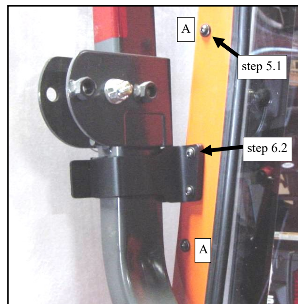
Fig. 5.1 (view of left side of tractor) (lower roll bar mount shown here)
