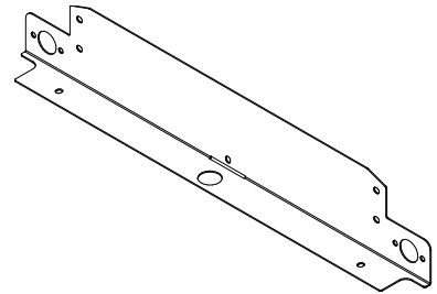
REAR LOWER CROSS P/N: 8SV-SM-01256
