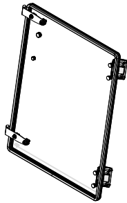
SIDE FRAME ASSEMBLY, LEFT P/N: 8SV-109-00024-L
