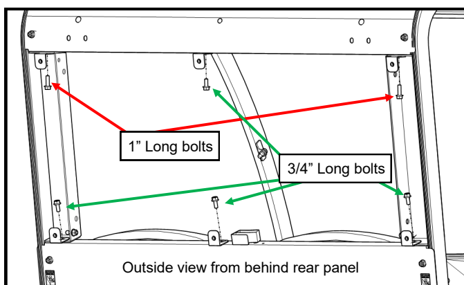
Figure 5.1: Rear Window Bracket Installation
