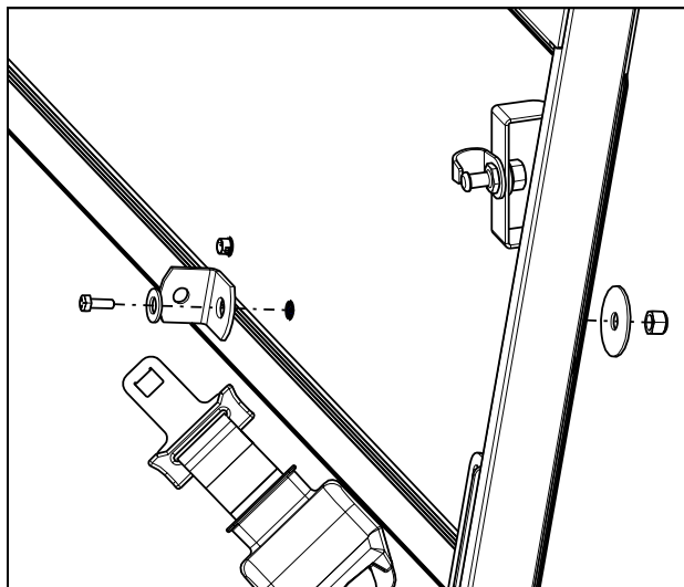
Fig. 9.5: Mounting bracket
