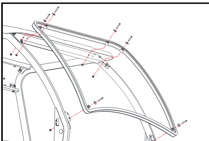
Figure 4.2: Windshield Installation
