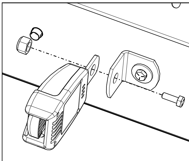
Fig. 9.6: Receiver Latch
