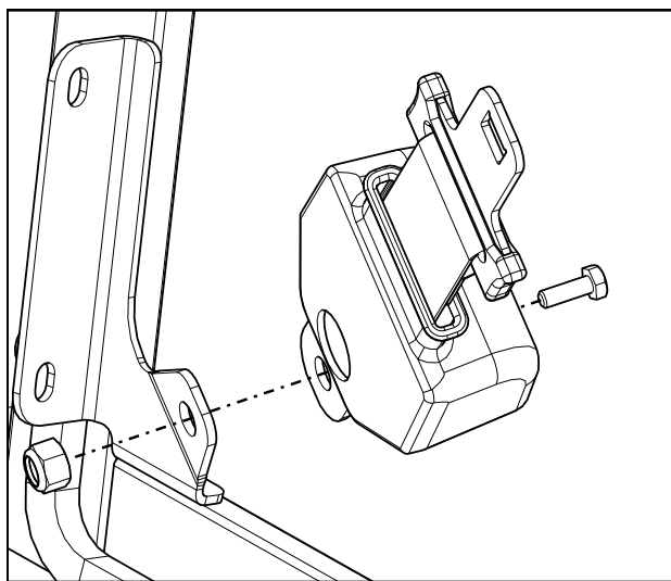
Fig. 9.3: Seat belt
