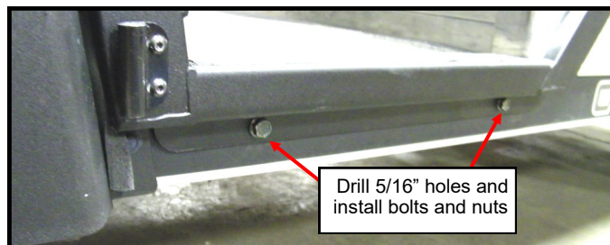
Figure 6.4: Floorboard bolts
