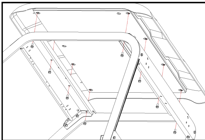
Figure 3.1: Roof Installation
