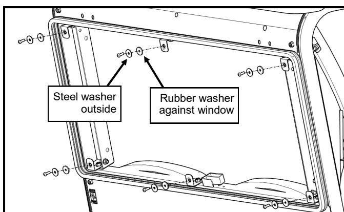
Figure 5.2: Rear Window Installation
