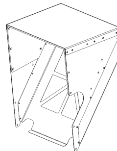
ROPS CLAMP, LEFT P/N: 8SV-110-00111-L
