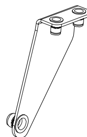
INNER FILLER BRACKET, RIGHT P/N: 8SV-110-00119-R
