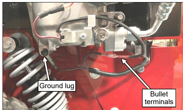
Fig. 6.7 (Compressor connections)
