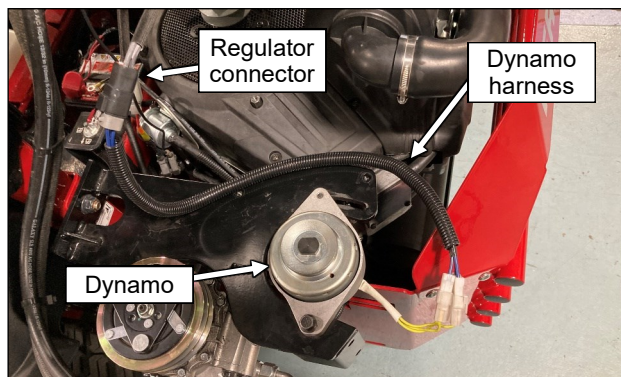
Fig. 6.9 (Dynamo connections)
