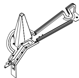
UNDER SEAT FILLER ASSEMBLY, RIGHT P/N: 8SV-111-00047-R
