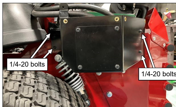
Fig. 9.1 (Compressor Debris Cover)
