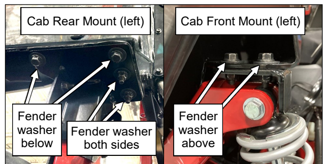
Fig. 4.8 (Cab mounting bolts)
