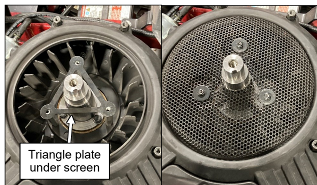
Fig. 1.6 (Re-install screen)
