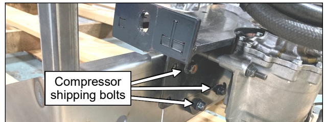
Fig. 4.3 (Unbolt Compressor)
