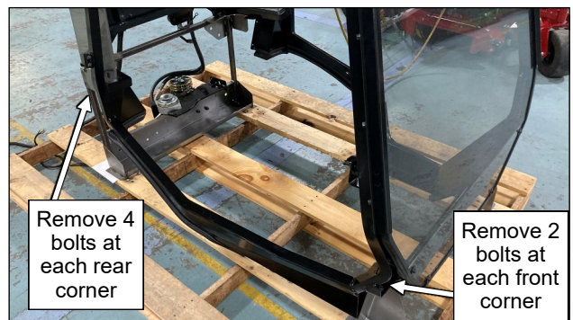
Fig. 4.5 (Cab pallet bolts)
