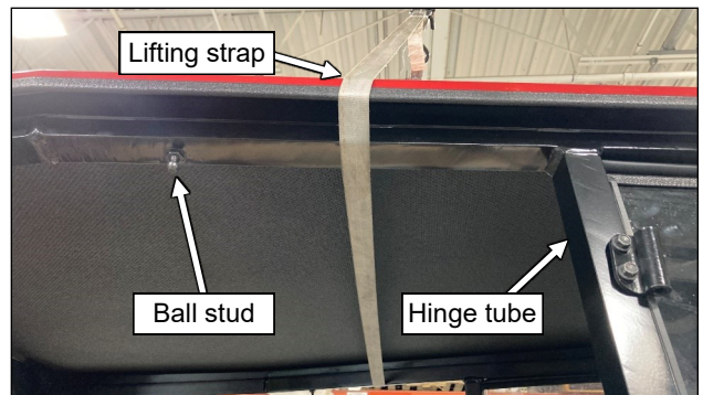
Fig. 4.4 (Position lifting strap)
