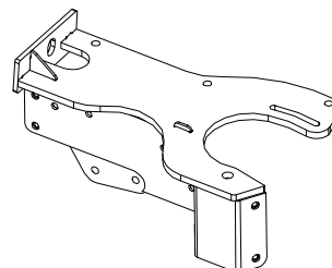
COMPRESSOR BRACKET P/N: 8SV-WA-00567
