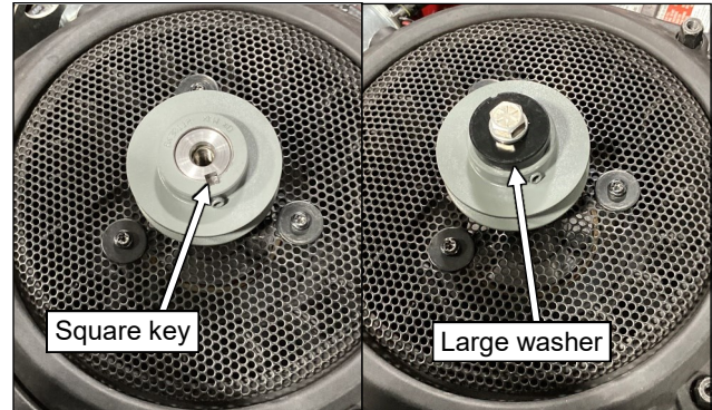
Fig. 1.7 (Install Pulley)
