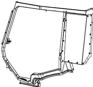
REAR BRACE ASSEMBLY P/N: 8SV-113-00298
