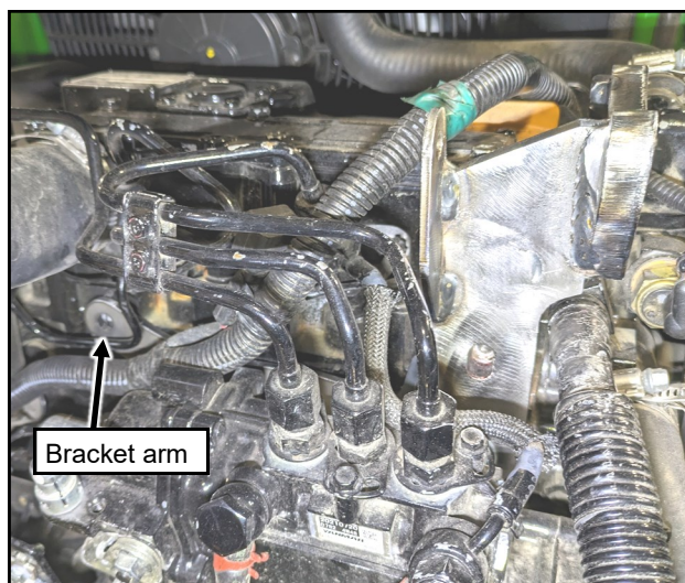
Fig. 1.36 (Snake compressor bracket into place)
