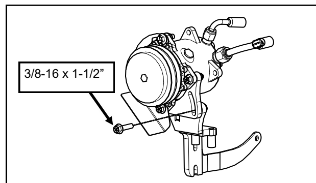
Fig. 2.11b (Install compressor)
