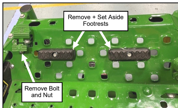
Fig. 1.13 (Remove Footrests & Brake Pedal Bolt)
