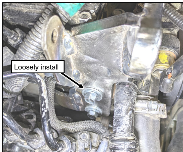
Fig. 1.37 (Loosely install second M8x1.25 x 25 screw)
