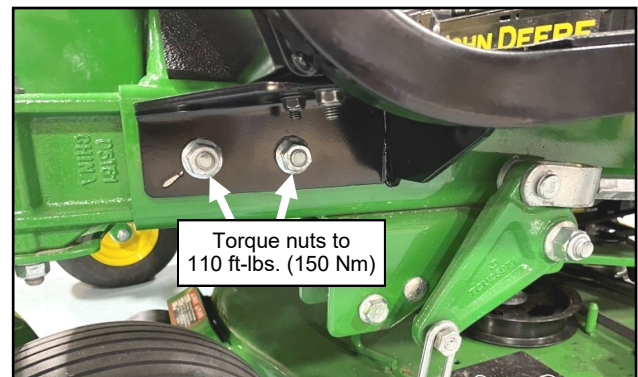
Fig. 2.9 (Tighten Vehicle Frame Bolts, Left)
