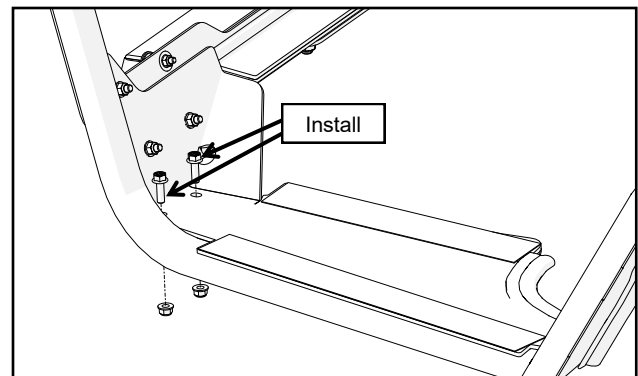
Fig. 2.8 (Install Front Mount Screws)
