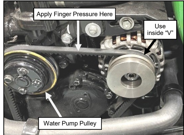
Fig. 1.7 (Install Double V-Pulley)
