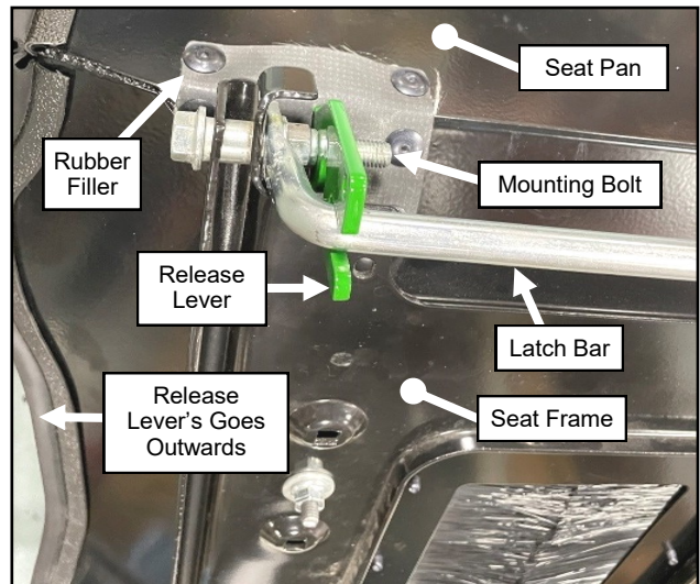
Fig. 1.26 (Install Seat Pan Assembly)
