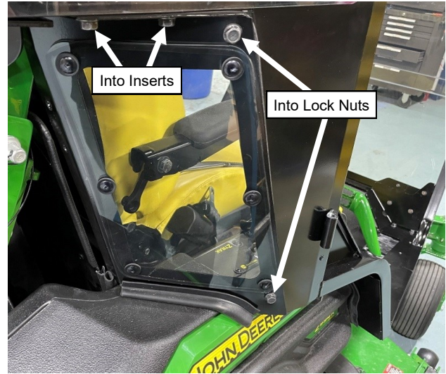
Fig. 2.15 (Install Right Filler)
