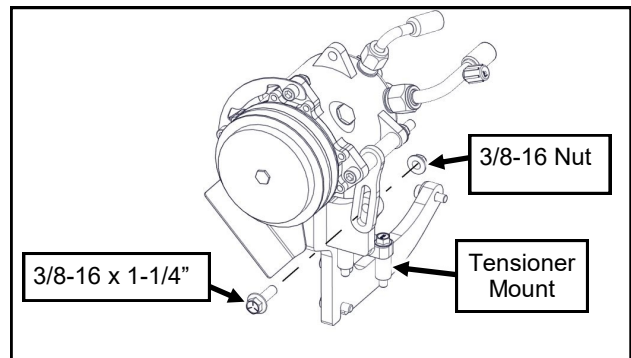
Fig. 2.11b (Install compressor)
