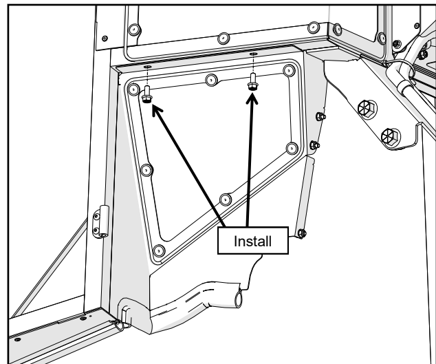
Fig. 2.16b (Install Left Filler, Outside View)
