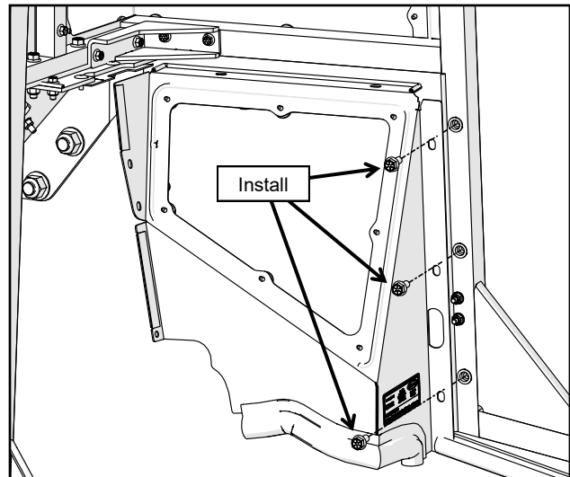
Fig. 2.16a (Install Left Filler, Inside View)
