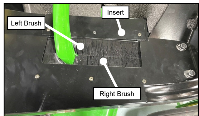
Fig. 2.10 (Install Brushes and Insert, Right)
