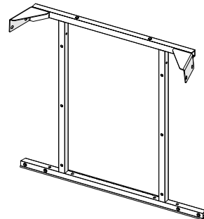
REAR MOUNT FRAME ASSEMBLY P/N: 8SV-113-00323
