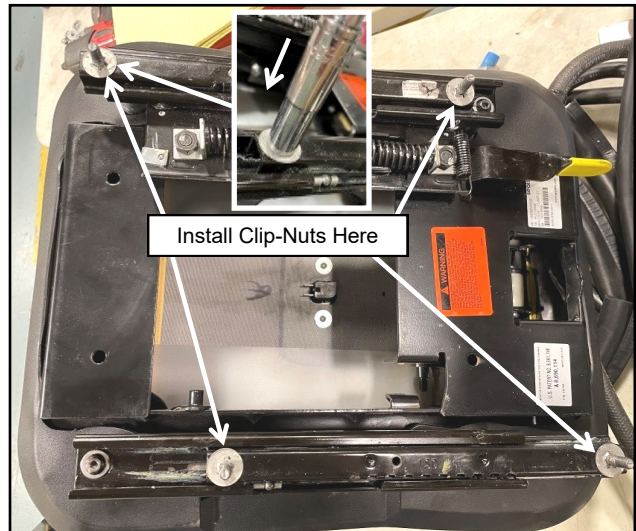
Fig. 1.25 (Install (4) Clip-On Nuts)
