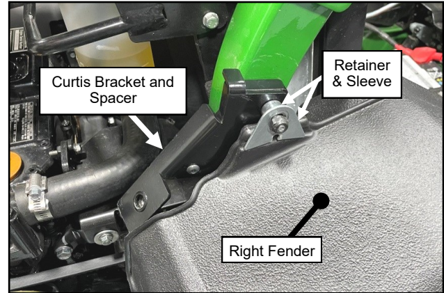
Fig. 1.11 (Install Bracket & Spacer)
