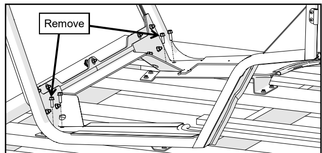
Fig. 2.4b (Remove Front Shipping Bracket Bolts)
