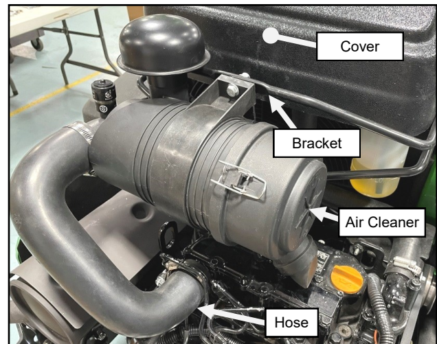
Fig. 1.8 (Remove Hose and Air Cleaner)
