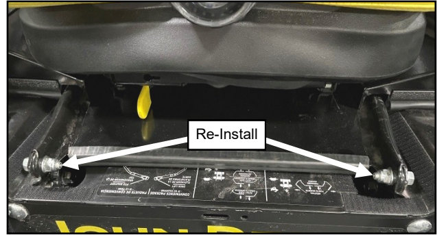
Fig. 1.28 (Re-Install Seat with Seat Pan)
