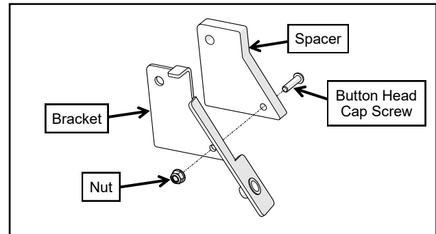
Fig. 1.10 (Install Spacer to Bracket)
