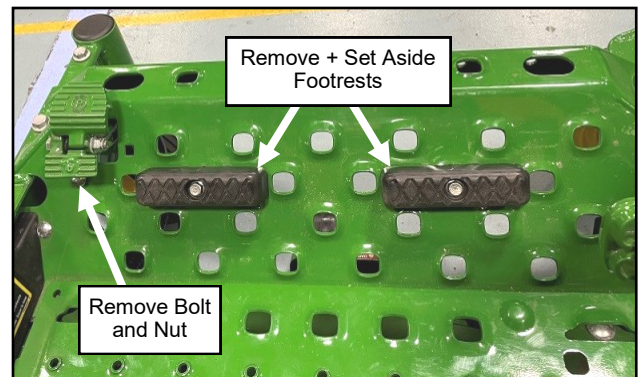
Fig. 1.13 (Remove Footrests & Brake Pedal Bolt)
