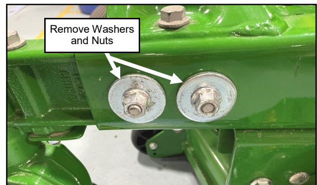
Fig. 1.14a (Remove M12 Washers and Nuts)
