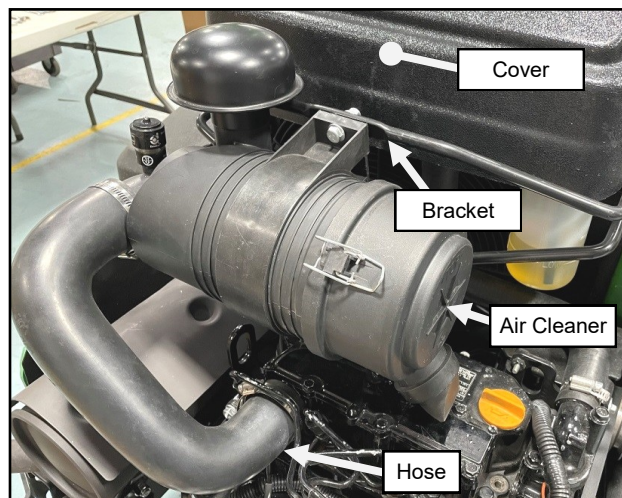
Fig. 1.8 (Remove Hose and Air Cleaner)
