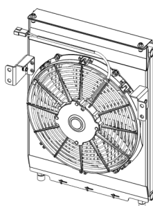
CONDENSER, PLENUM & FAN, BLACK P/N: 8SV-304-00027-BP
