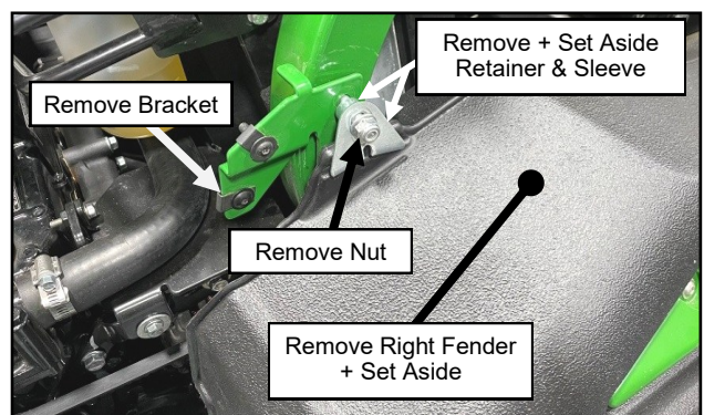
Fig. 1.6 (Remove Right Fender)
