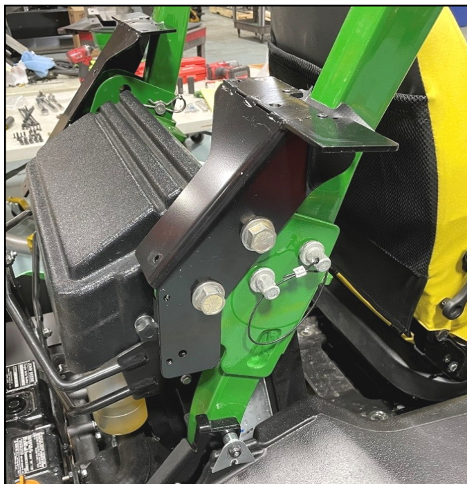
Fig. 1.30b (Install R.O.P.S bracket, right)
