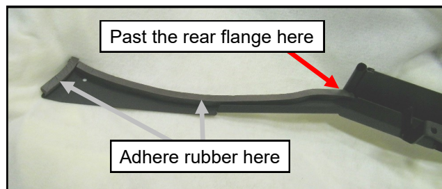
Fig. 6.2 (C-pillar foam rubber)
