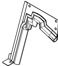
LEFT FENDER FILLER PANEL P/N: 8SV-111-00055-L
