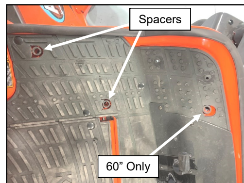
Fig. 4.7 (Install Spacers)
