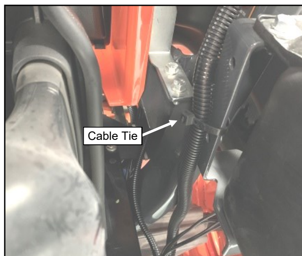
Fig. 7.6 (Secure Wire Harness)
