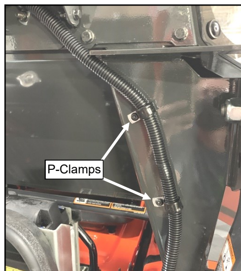
Fig. 7.5 (P-Clamp Wire Harness to ROPS Bracket)
