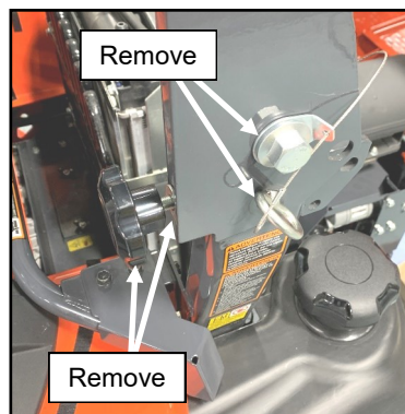
Fig. 3.1 (Remove hand screws and ROPS Bolt)
