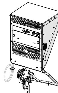
CONDENSER SUPPORT ASSEMBLY, BLACK P/N: 8SV-304-00029-BP
