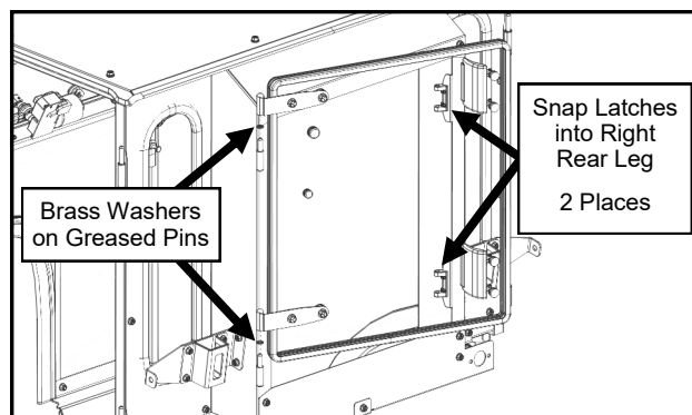
Fig. 16.2 (Hang Rear Window)
