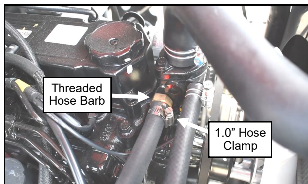
Figure 20.6 (Install Threaded Hose Barb Nipple)
