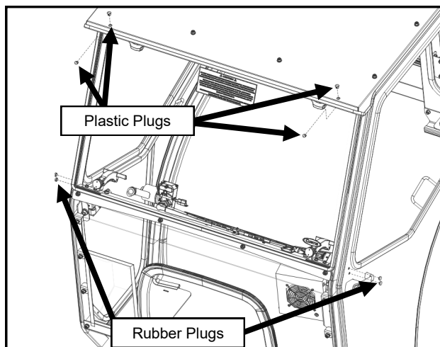
Fig. 26.1 (Install Plugs)
