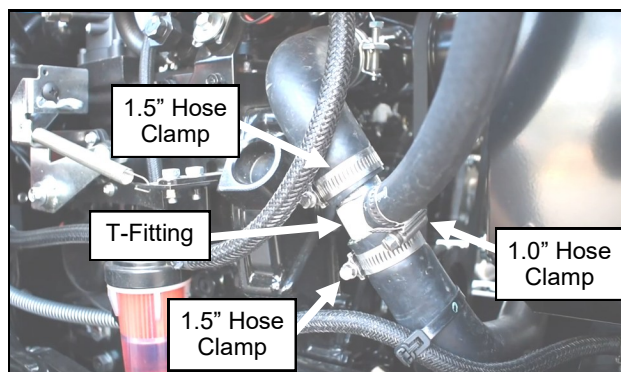
Figure 20.5 (Install T-Fitting in Lower Hose)
