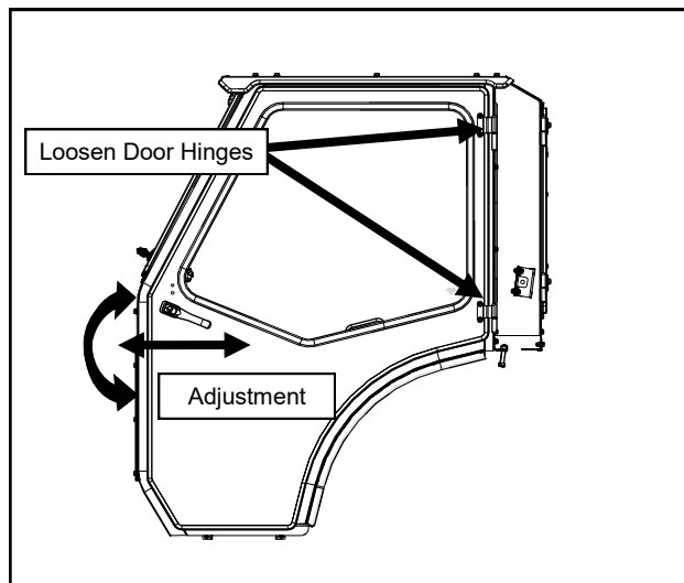
Fig. 25.2a (Door Hinge Adjustment)
