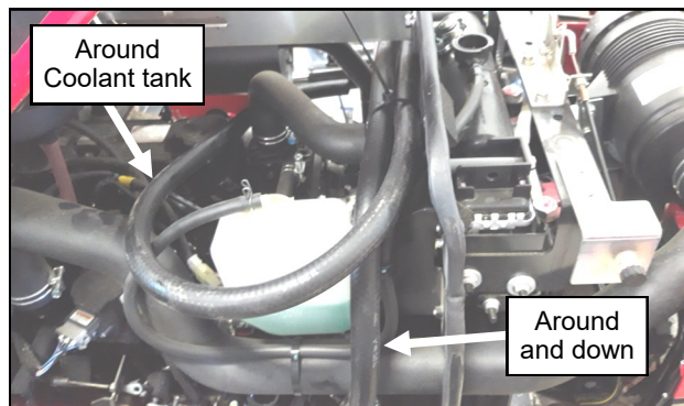
Figure 20.3 (Right Side of Engine Bay)
