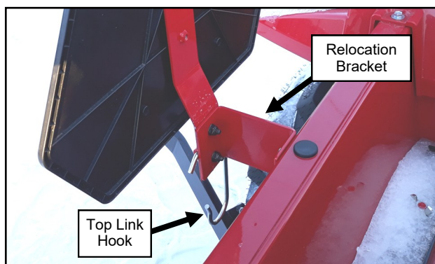
Fig. 26.3 (Install SMV Sign and Top Link Hook)
