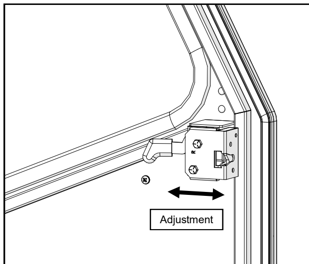
Fig. 25.2c (Door Latch Adjustment)
