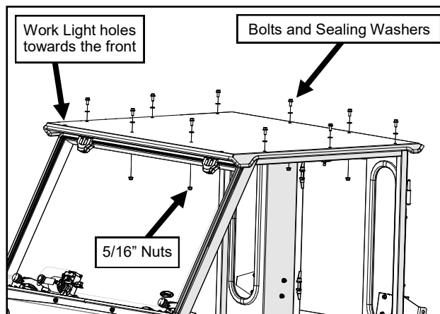
Fig. 15.2 (Install Roof)
