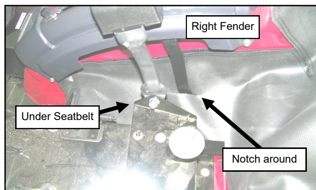
Fig. 24.4b (Install Under Seat Filler)
