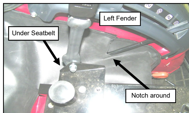
Fig. 24.4a (Install Under Seat Filler)
