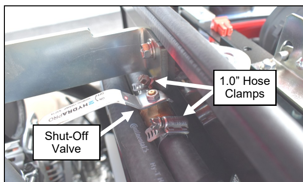
Figure 20.8 (Install Shut-Off Valve)
