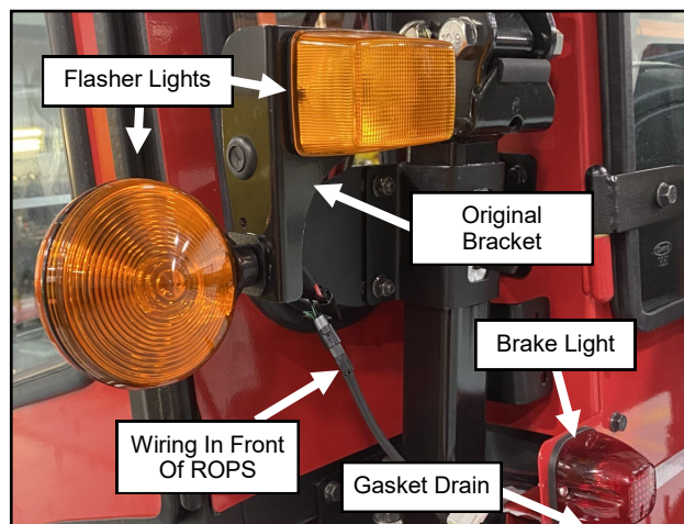
Fig. 23.1 (Mount Rear Lights)
